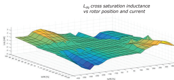
Inductance and flux parameters for sensorless drive.
