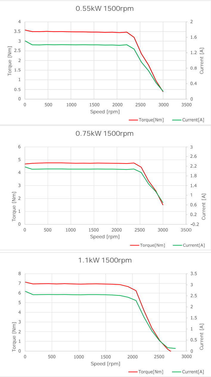
Performance Graphs for 80 Frame Motors
